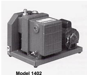
Model 1402 Displacement 5.6 CFM Ultimate Pressure .0001 Torr
