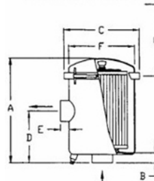
2" to 2 1/2" Connection
